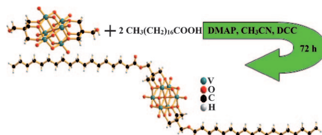
Figure 1. Synthesis of 1 2- . DCC = 1,3-dicyclohexylcarbodiimide, DMAP = 4-dimethylaminopyridine.
